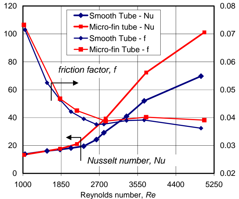
Figure 2: Nusselt number and friction factor vs. Re .
